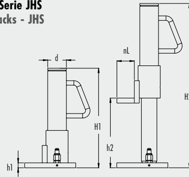
Schieber 180° schwenkbar 180° revolving housing
